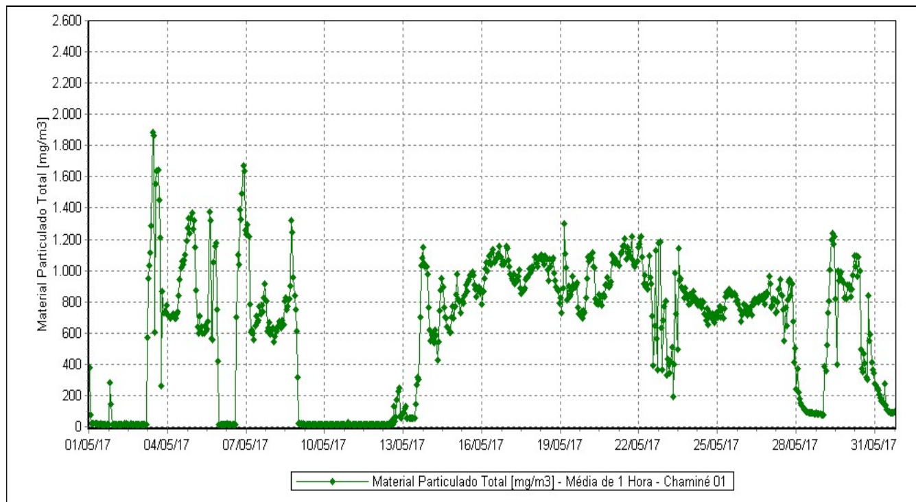
Figura 4. Material Particulado Total [mg/m 3 ] – Chaminé 1
